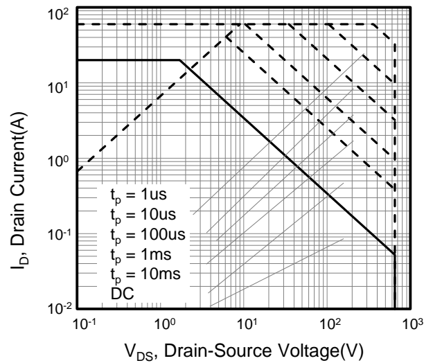
Figure 10. Safe Operation Area For TO-220F/TO-220FP-NL
