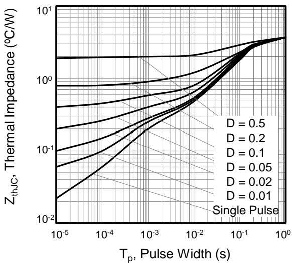
Figure 9. Transient Thermal Impedance For TO-220F/TO-220FP-NL
